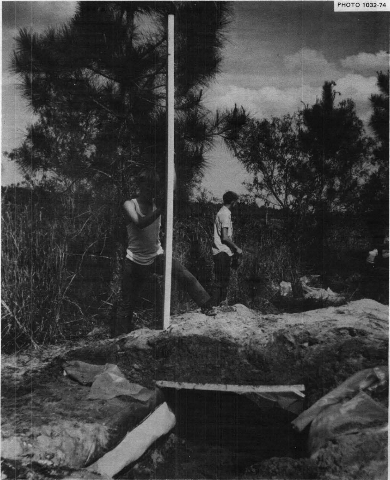
Fig. 5.60. The painted hollow-core door previously pictured, soon after it had been uncovered and removed from the walls made of rolls. Note how slight was its permanent warp or bow. The second painted door is pictured in test position.
